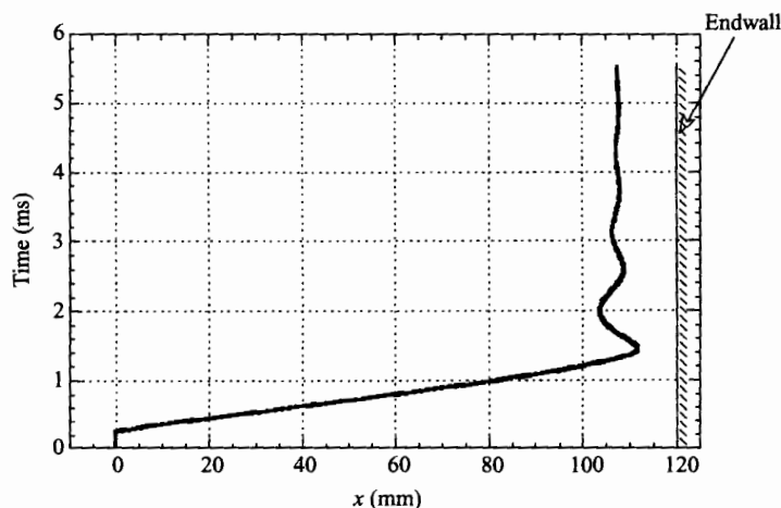
FIGURE 7. The calculated time-dependent trajectory of the foam/gas interface. It is seen, immediately following the head-on collision, to move at a nearly constant velocity, in full agreement with experimental results (see e.g. Ben-Dor et al. 1994), until the foam reaches a maximum deformation of about 92%. The constant velocity of the front edge of the foam is about 100 \text{ m s}^{-1} . This value is close to those measured in similar experiments.
