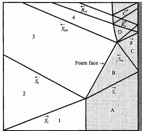
FIGURE 3. A simple refraction-model-based wave diagram of the head-on interaction of a planar shock wave with a flexible porous medium, which was accepted as the state-of-the-art until the early 1990s.
