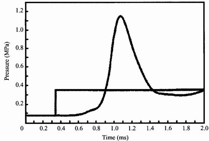
FIGURE 5. The pressure enhancement phenomenon at the shock tube endwall as recorded experimentally by Skews et al. (1993). The straight-line stepped trace is the theoretical prediction with no foam present. The pressure behind the head-on reflected shock wave for a rigid wall reflection is constant at about 350 kPa compared to a maximal pressure of about 1150 kPa for the case of a head-on reflection in the presence of the foam.
