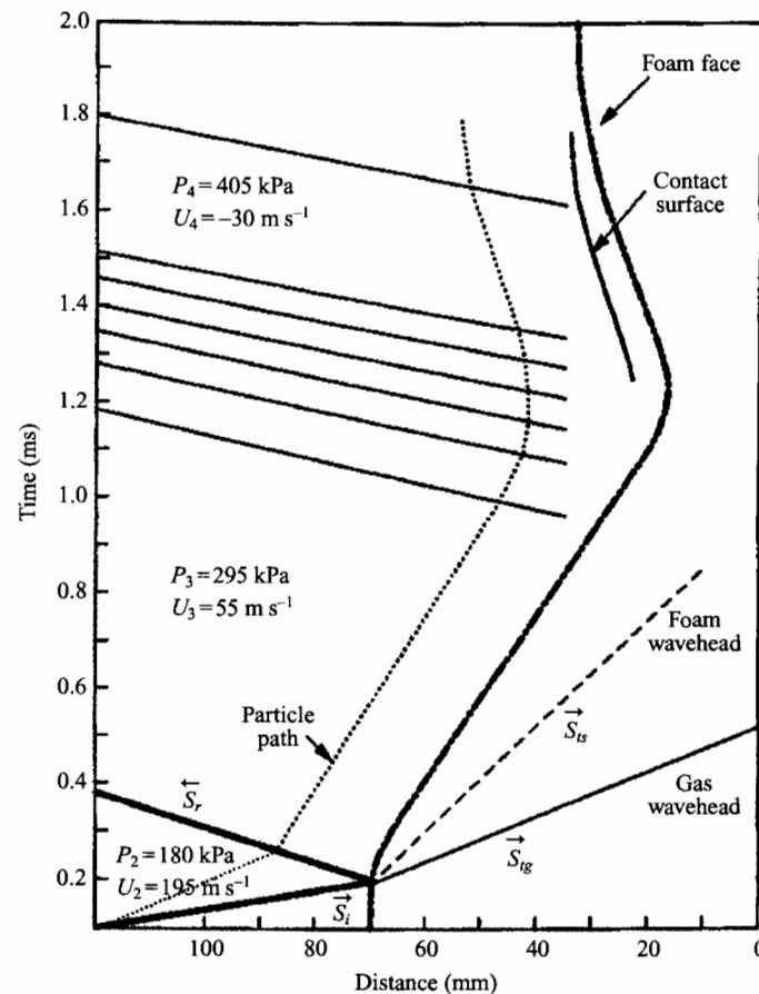
FIGURE 4. An innovative wave diagram of the head-on interaction of a planar shock wave with a flexible porous medium, as proposed by Skews et al. (1993) following their comprehensive experimental study, which revealed that the wave diagram shown in figure 3 is over-simplified since it considers the foam as a single phase while it actually consists of at least two phases (i.e. the solid skeleton and the gas that occupies the pores).
