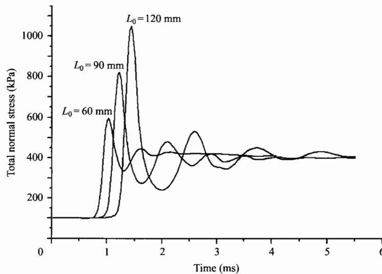
FIGURE 11. The dependence of the pressure enhancement on the length of the foam. The peak pressure increases as the length of the foam increases while the shape of the pressure pulse at the shock tube endwall remains similar. This behaviour is in full agreement with the available experimental results (see e.g. figure 6).
