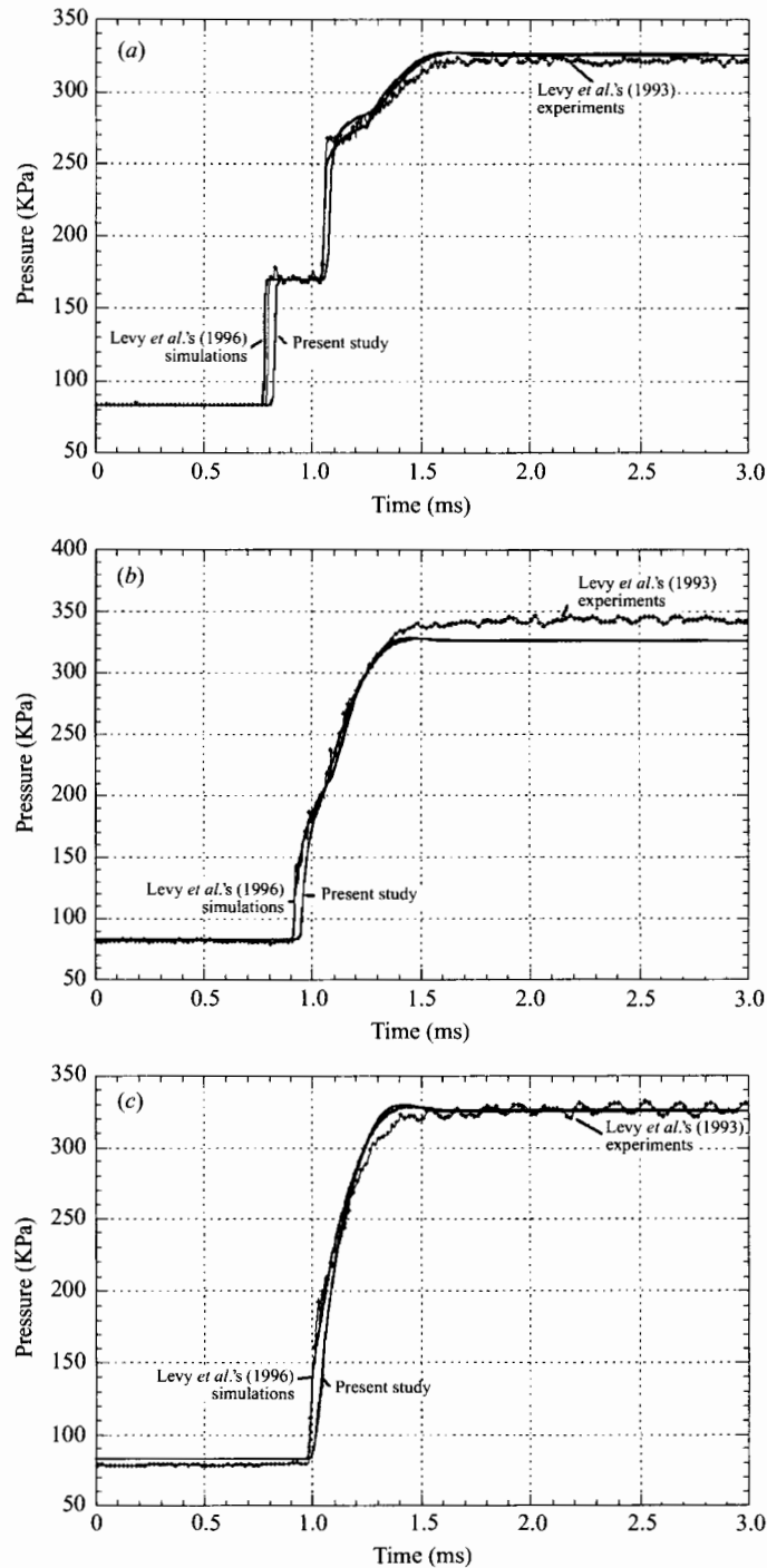
FIGURE 1. Typical experimental results and numerical simulations with a 40 mm long sample made of silicon carbide (SiC) which has 10 pores per inch and average porosity 0.728 \pm 0.016 . The incident shock wave Mach number in this experiment was M_s = 1.378 . (a) The pressure history of the pure gas 43 mm ahead of the front edge of the porous material. (b, c) The pressure histories of the gas occupying the pores of the porous material along the shock tube sidewall (23 mm from the endwall) and at its endwall respectively.
